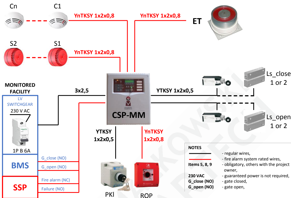
Fig. 4 – MARC-O control system with electromagnetic holder
