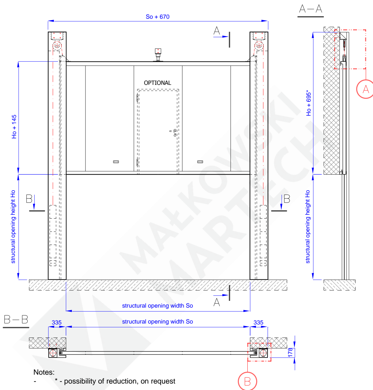
Fig. 1 – Fire protection vertically sliding door MARC-O EI60
