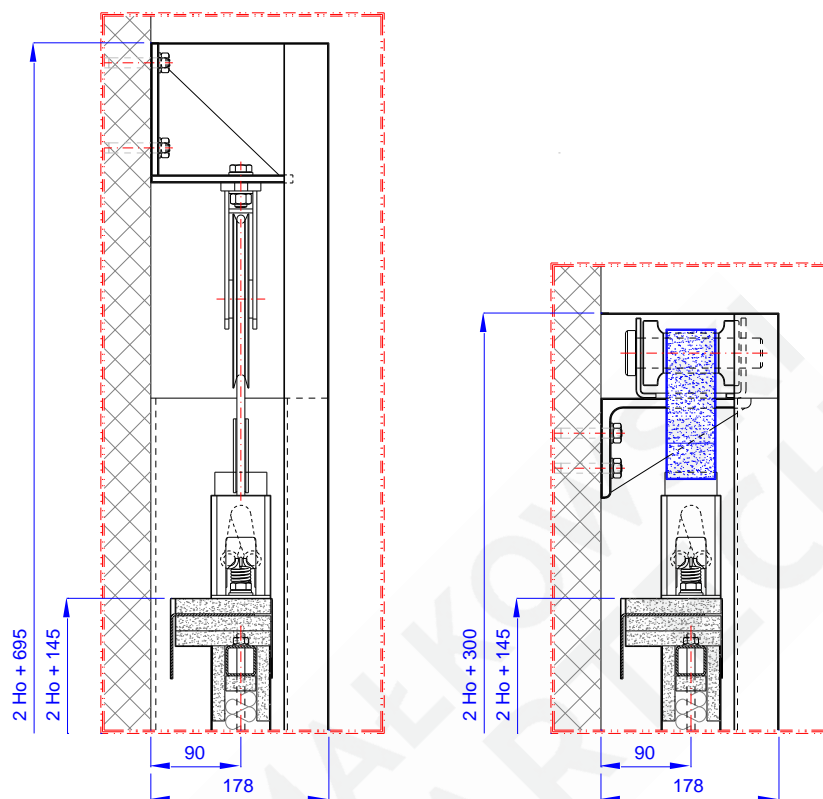
Fig. 2 – Detail A from Fig. 1 – variant with the cables on the left and with the belts on the right side
